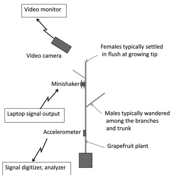
Fig. 1. Experimental arena inside the vibration-shielded anechoic chamber. Video monitor, laptop controller, and the vibration analysis and recording system were external to the chamber.
