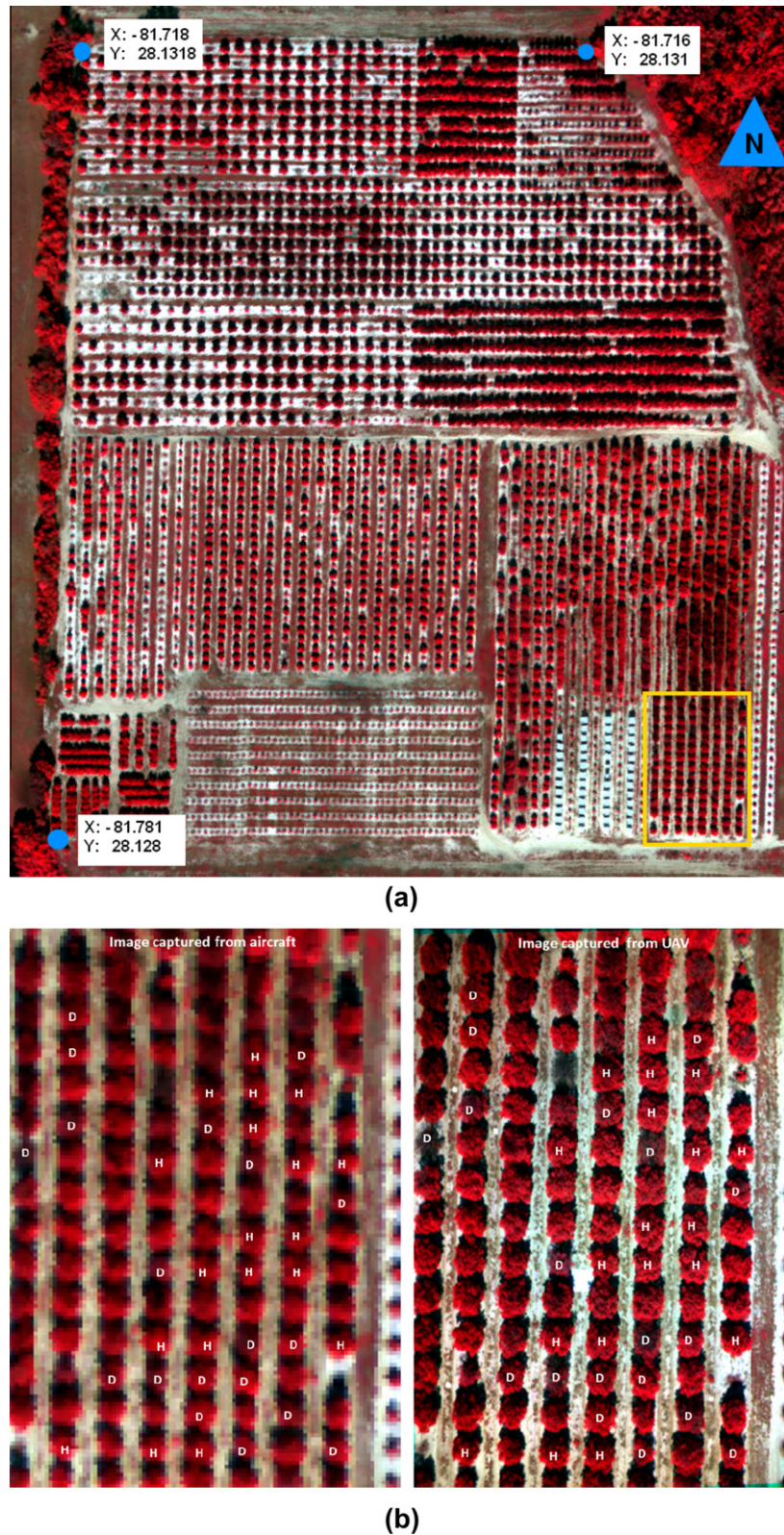
Fig. 2. (a) False color image of the study area with marked region of interest (ROI); (b) Aerial images with marked Healthy (H) and HLB-infected trees (D) within the ROI as acquired from aircraft (left) and UAV (right).
