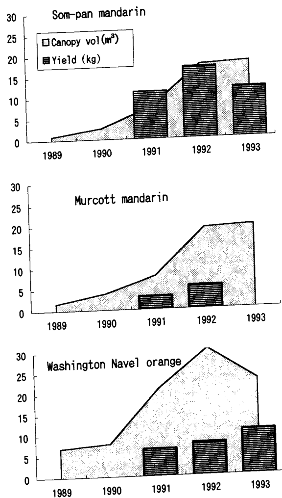
Fig. 3. Annual changes in canopy volume and yield of sweet orange and mandarin trees planted in a HGB-infected field
