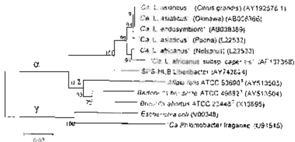
Fig. 4. Phylogenetic tree constructed with MEGA version 2.1 using 118 rDNA sequence. (GenBank accession numbers in parentheses).
