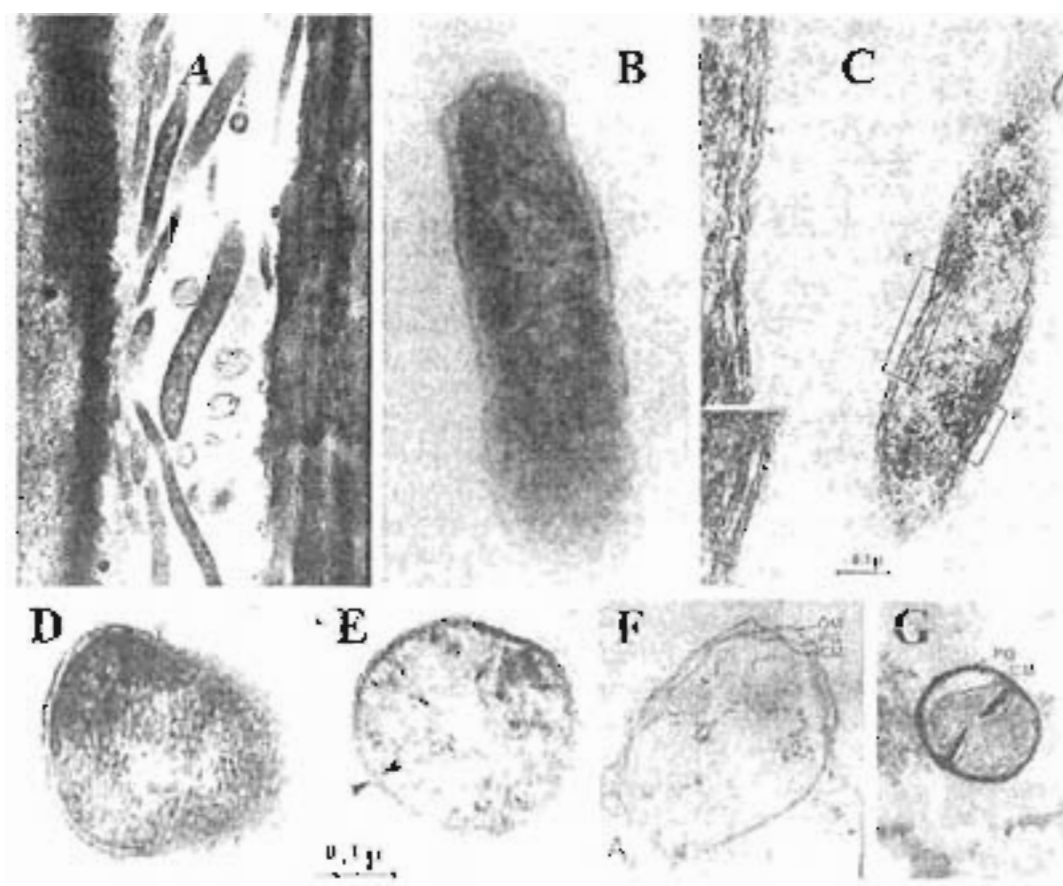
Fig. 3. Electron micrograph of liberibacter cells in a sieve tube of sweet orange leaf (Saudi Arabia) (A). At higher magnification, the cells are seen surrounded by a cell wall, which shows up as an electron dense layer (B, D). At even higher magnification and with special techniques, one sees the triple-layered ultrastructure of both the outer cell wall membrane and the inner cytoplasmic membrane (C: \rightarrow \rightarrow \rightarrow ), while mycoplasmas, such as Spiroplasma citri seen here (E: \rightarrow \rightarrow ) have no cell wall, and are surrounded by a cytoplasmic membrane only. With special techniques, the peptidoglycane layer of the Gram negative cell wall can be visualized (F: \rightarrow on F) in between the inner membrane cytoplasmic membrane (CM on F) and the outer cell wall membrane (OM on F). The cell wall of Gram positive bacteria has no membrane, but only a heavy layer of peptidoglycane (PG on G), surrounding the cytoplasmic membrane (CM on G). All electron micrographs are from M. Garnier.
