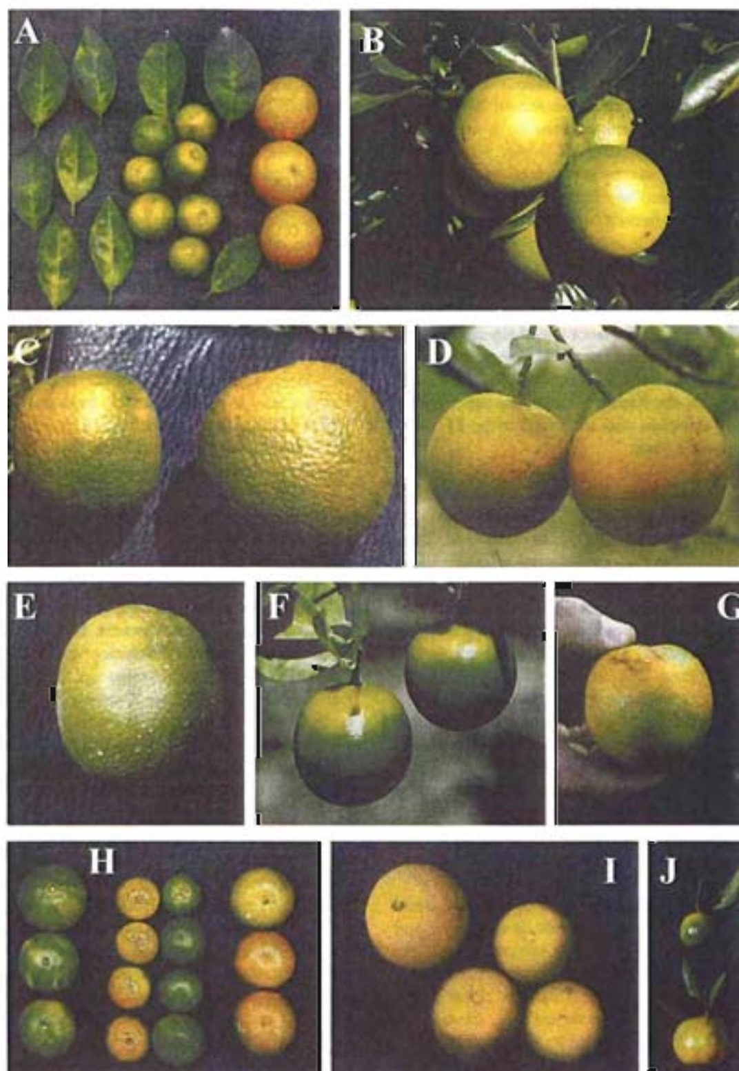
Fig. 9. The two most characteristic symptoms of HLB are leaves with blotchy mottle and fruits with small size and colour inversion (A, normal sweet orange on right; Beihai, Guangxi, China). Poorly coloured "greening"-affected oranges from South Africa (C), which, when pressed with a finger, develop a silvery "finger mark" (E). Normal oranges with coloration starting at the stylar end (B). Oranges and mandarins with coloration starting at the peduncular end (colour inversion) (i) sweet oranges from China, Guangxi (D) and Fujian (H, normal fruits with orange stylar ends on far right, and green peduncular ends on far left; fruits with colour inversion, in the middle), and São Paulo State, Brasil (G, I); (ii) mandarins from North Bali (F), and China (J, lower fruit: normal, upper fruit: with colour inversion).
