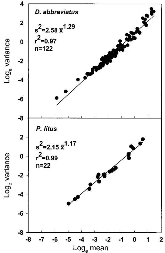
Fig. 2. Relationships between variances and means (weevils/trap/mo) of the numbers of (A) Diaprepes abbreviatus from six citrus groves, and (B) Pachnaeus litus from two citrus groves.
