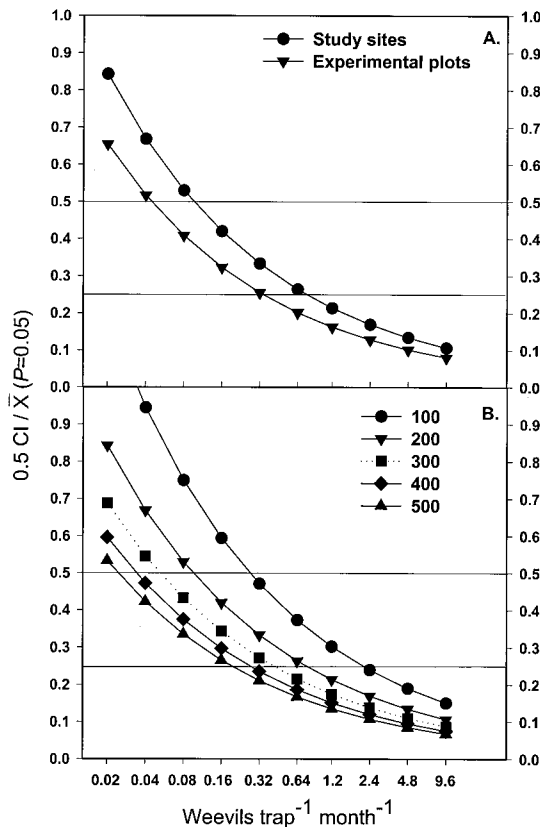
Fig. 3. Predictions of the precision with which Tedders traps will measure the mean density of Diaprepes abbreviatus using Taylor's power law in the equation 0.5 CI / \bar{X} = \sqrt{z_{\alpha/2}^2 a \bar{x}^{b-2} / n} for (A) plots of different size (0.06–0.46 ha versus 1.6–12.6 ha) using 200 traps and (B) large plots using different numbers of traps. Parameters for small plots were a = 1.56 , b = 1.32 , and for large plots a = 2.69 , b = 1.33 .
