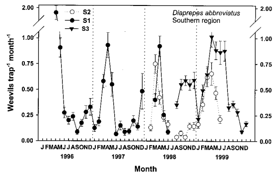
Fig. 5. Mean and standard error of numbers of Diaprepes abbreviatus trapped monthly in three citrus groves in the southern region of the Florida citrus industry. Numbers of weevils trapped at the S3 site were divided by 4.0 to facilitate comparison of sites.
